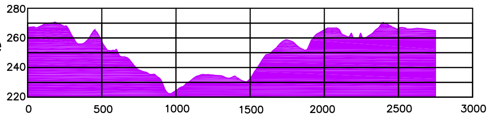
Profile Scale Horizontal 1:25000 Vertical 1:2500
